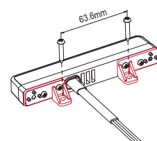
L-Bracket (Rear)
