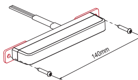
L-Bracket (Front)
